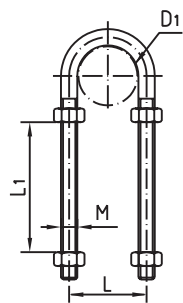
Rohrspannbügel DIN lang pipe support
